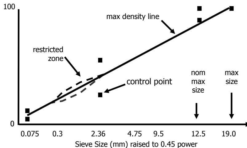
Figure 4: Aggregate blend gradation chart with Superpave gradation limits
