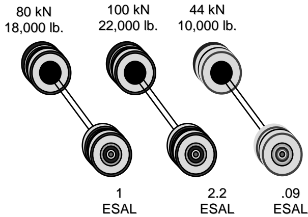
Figure 1: ESAL comparison
