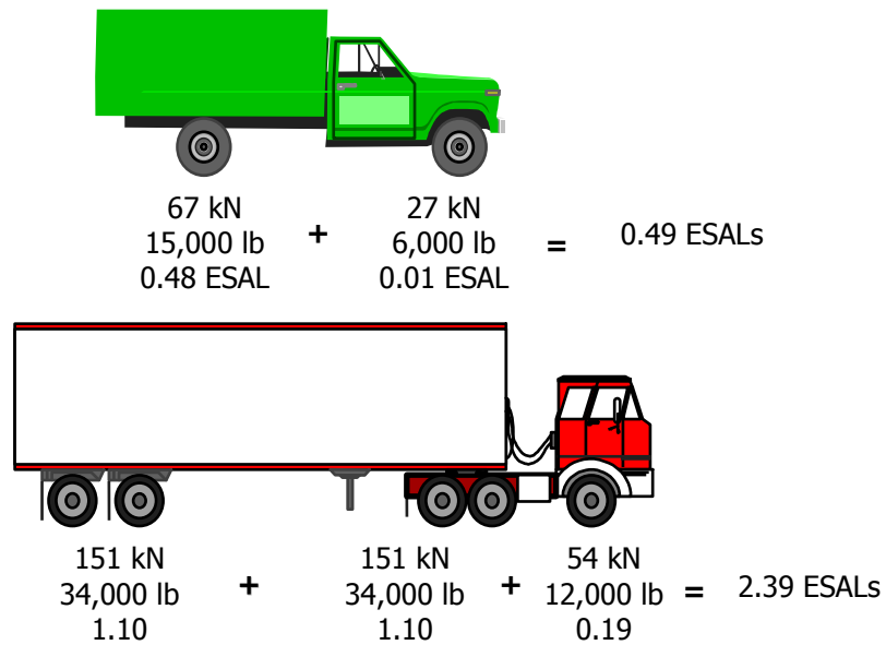
Figure 2: Example ESALs calculation
