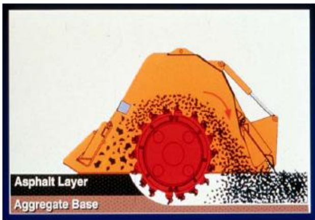
Figure 1. Graphic of the In-Place Recycling Process. (Graphic courtesy of ARRA)
